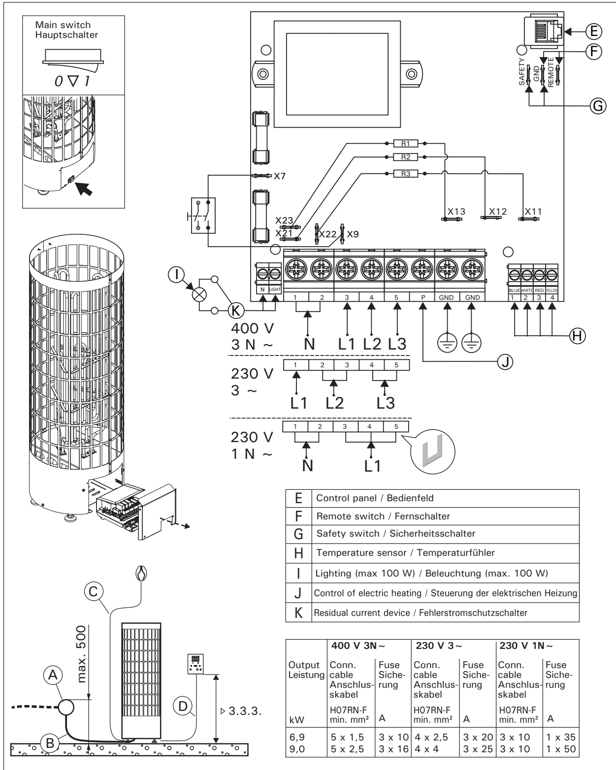
Figure 7. Electrical connections Abbildung 7. Elektroanschlüsse
