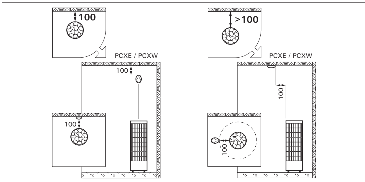
Figure 8. Installing the sensor (all dimensions in millimeters)
