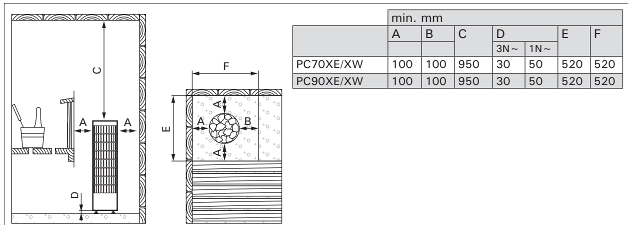
Figure 6. Safety distances (all dimensions in millimeters)
