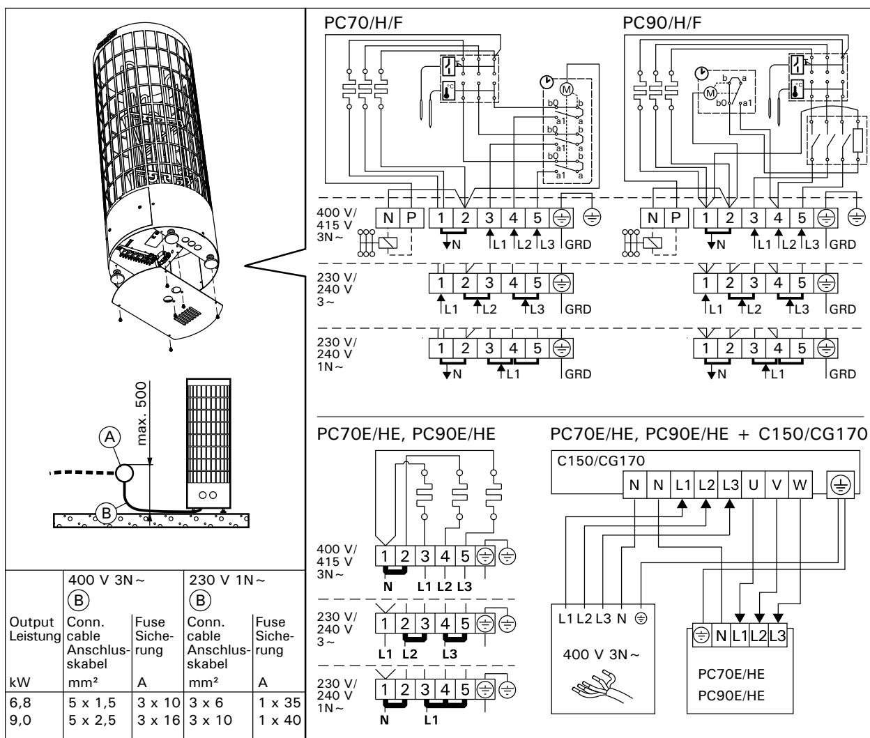
Figure 7. Electrical connections Abbildung 7. Elektroanschlüsse
